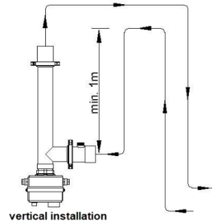
vertical installation
