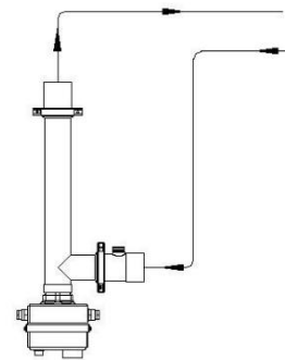
vertical installation
